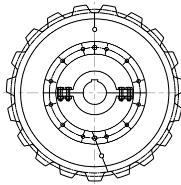
SPLIT SPROCKET WITH REPLACEABLE SEGMENTS
