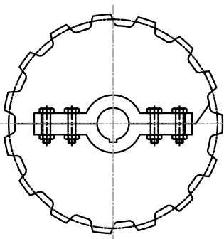
SPLIT SPROCKET-DRIVE
